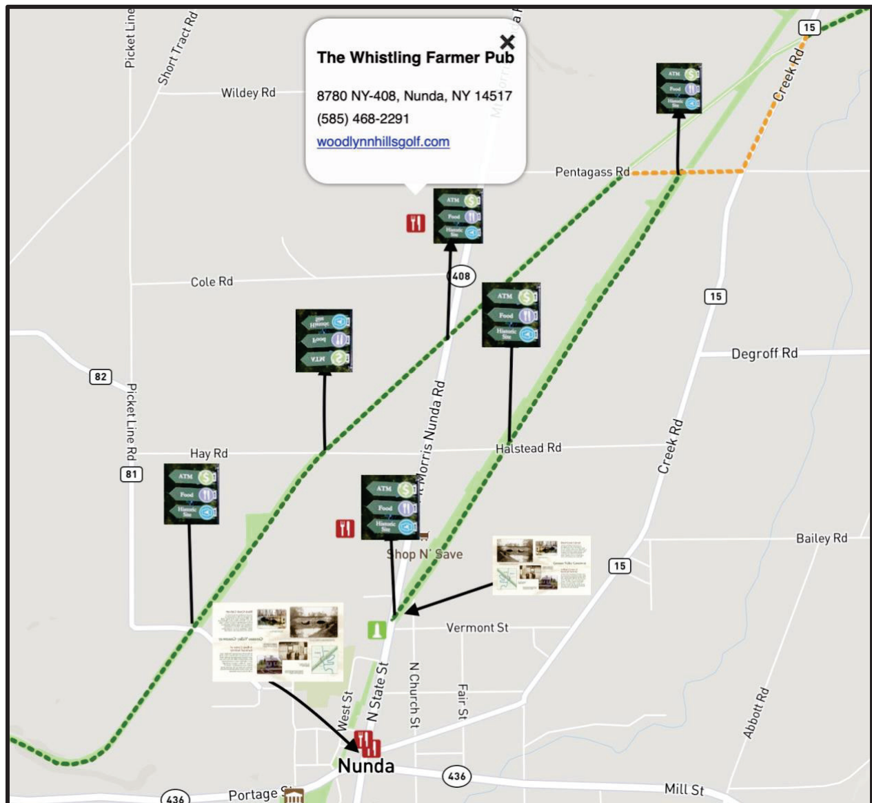
Location of proposed Wayfinding Signs. Three (3) signs on main Greenway Trail, two (2) on GVG Branch Trail, and one (1) at GVG Branch Trailhead.
